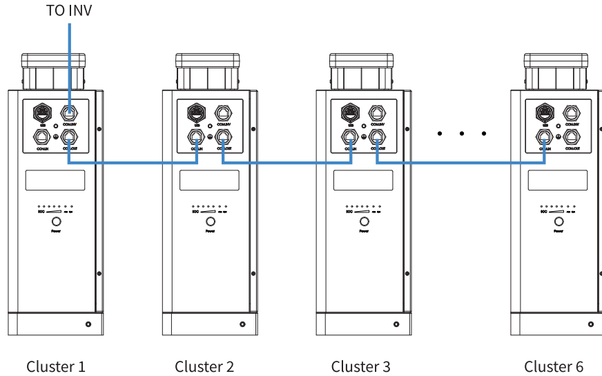
Multi-cluster communication wiring
